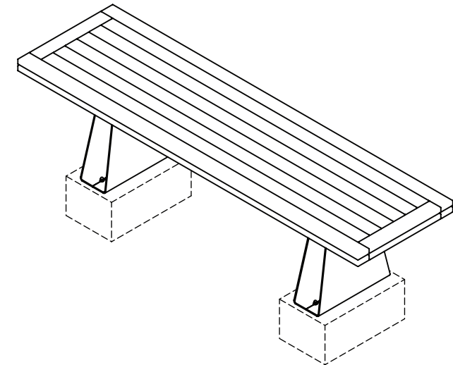
ISOMETRIC VIEW (SCALE 1:30)
