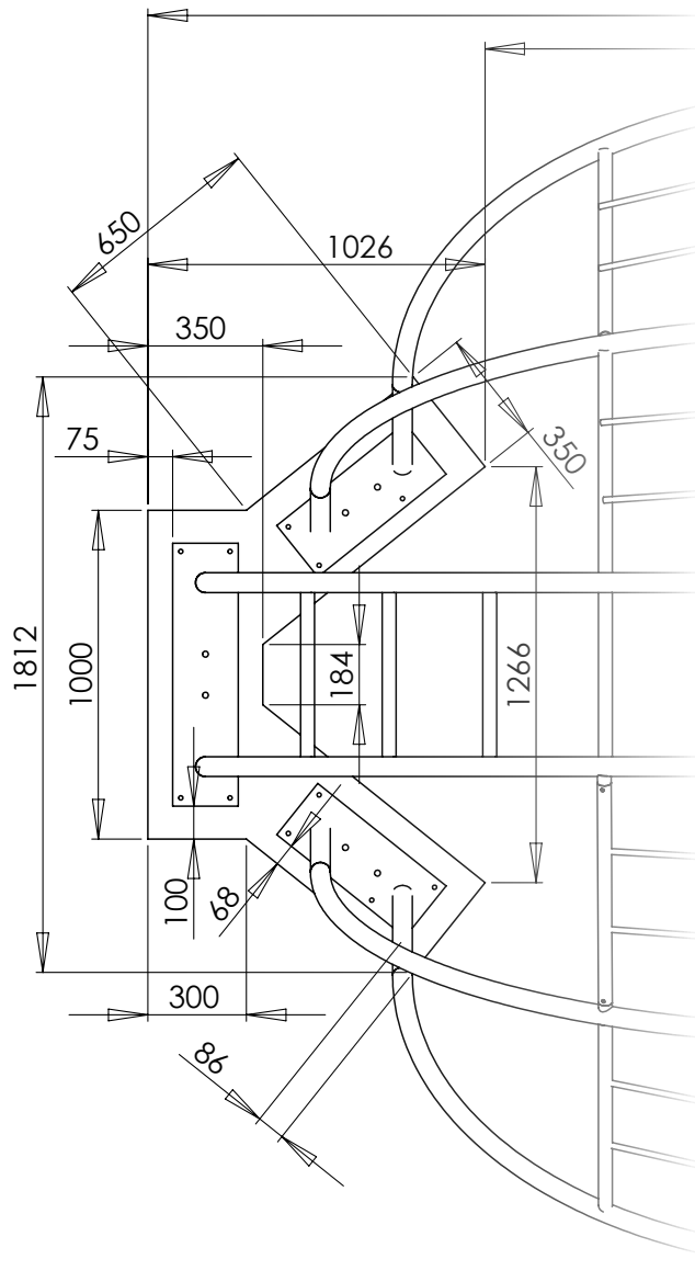
Diagramm 3b: Rear view foundationplan
