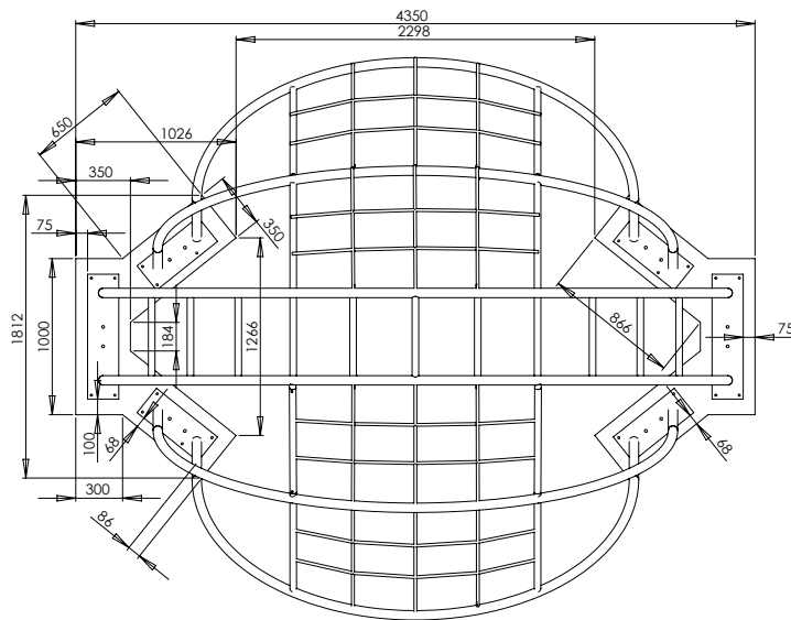
Diagramm 3a: Top view foundationplan
