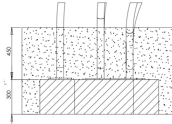
Diagramm 3b: Rear view foundationplan
