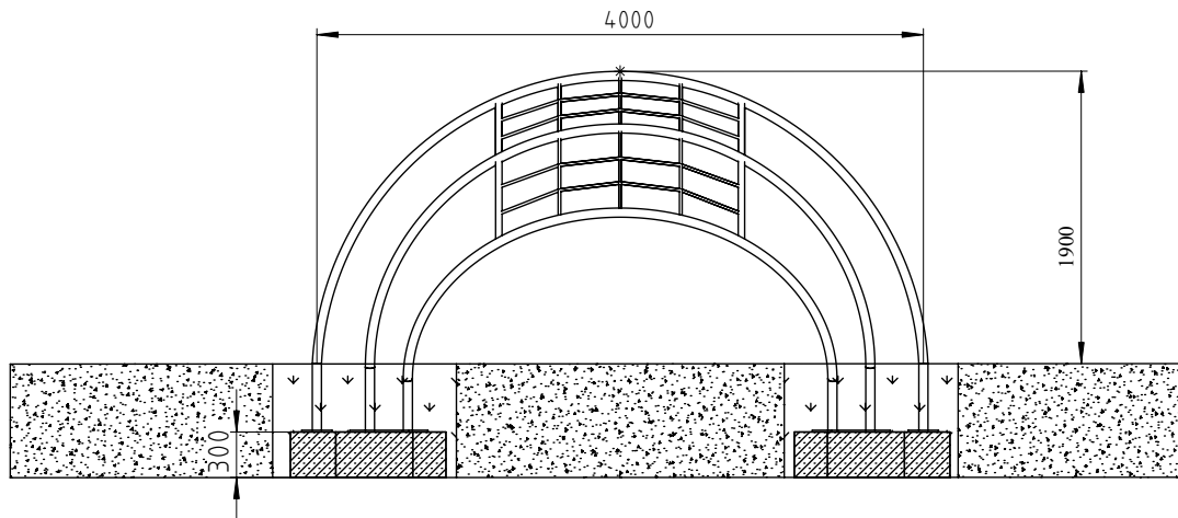
Diagramm 2: Rear view with dimension details „collis“
