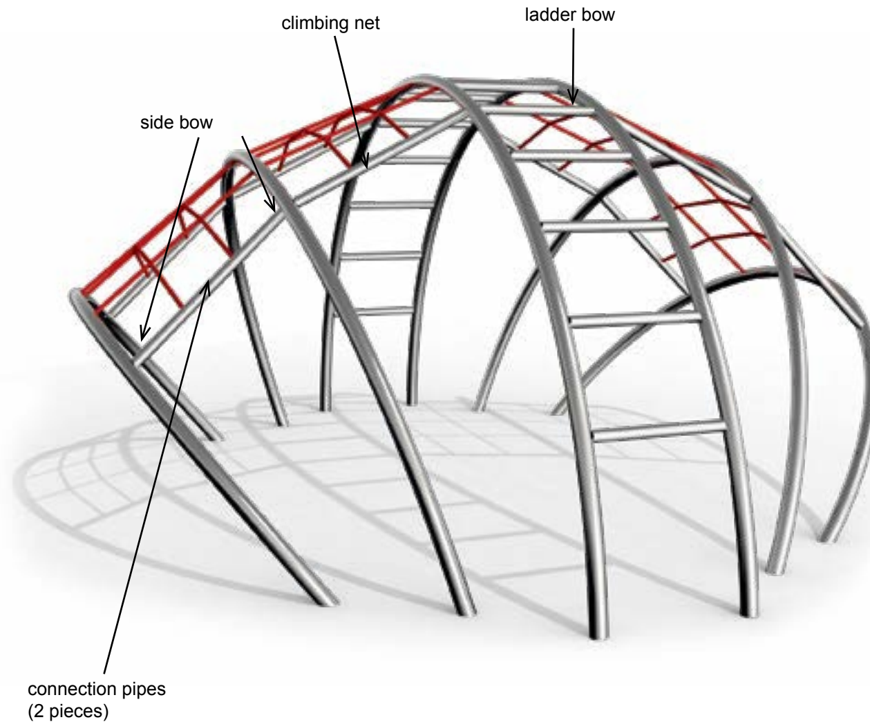
Diagramm 1: Overall view play equipment with description of individual elements
