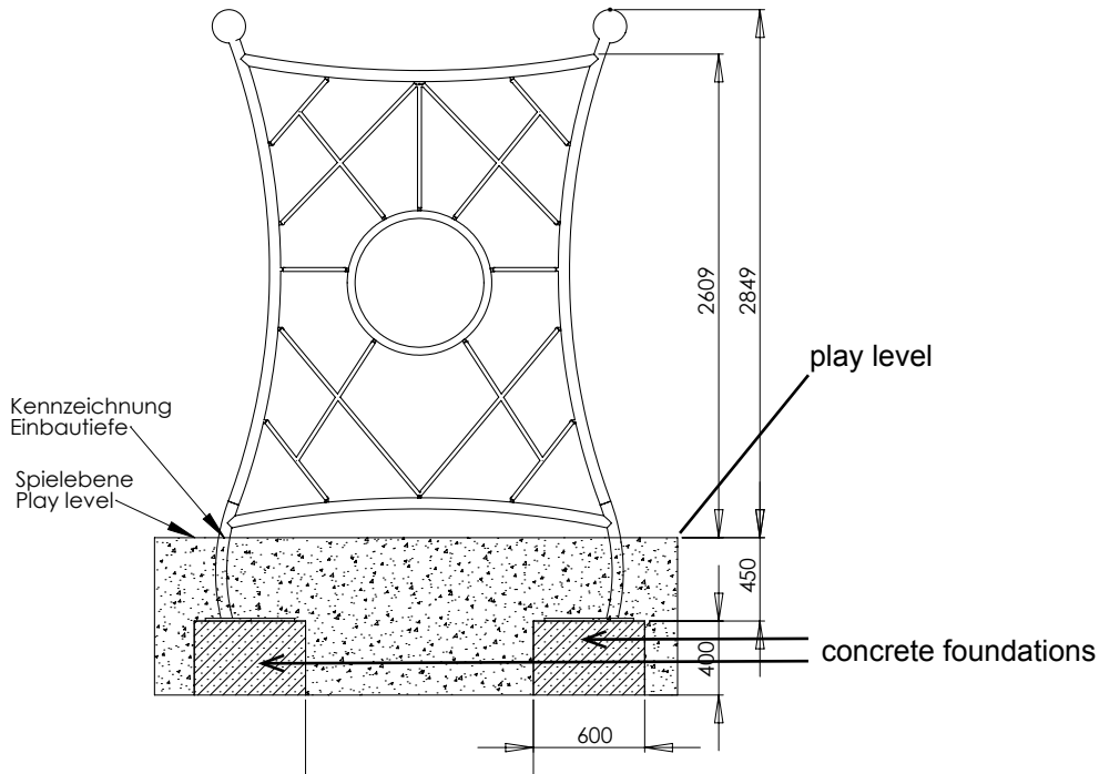
Diagramm 2: Rear view with dimension details „retis 2“
