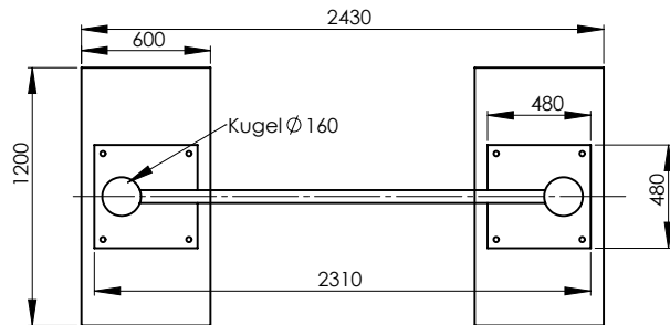
Diagramm 3: Top view foundationplan
