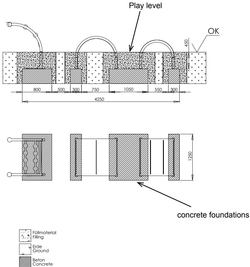
Diagram 2: Side view with dimension details „Erika“
