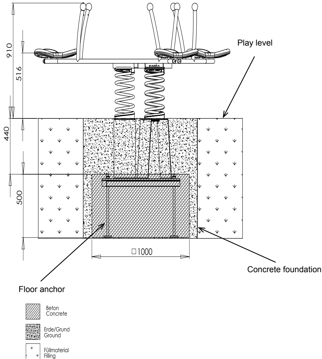
Diagram 2: Side view with dimension details „papilio3“
