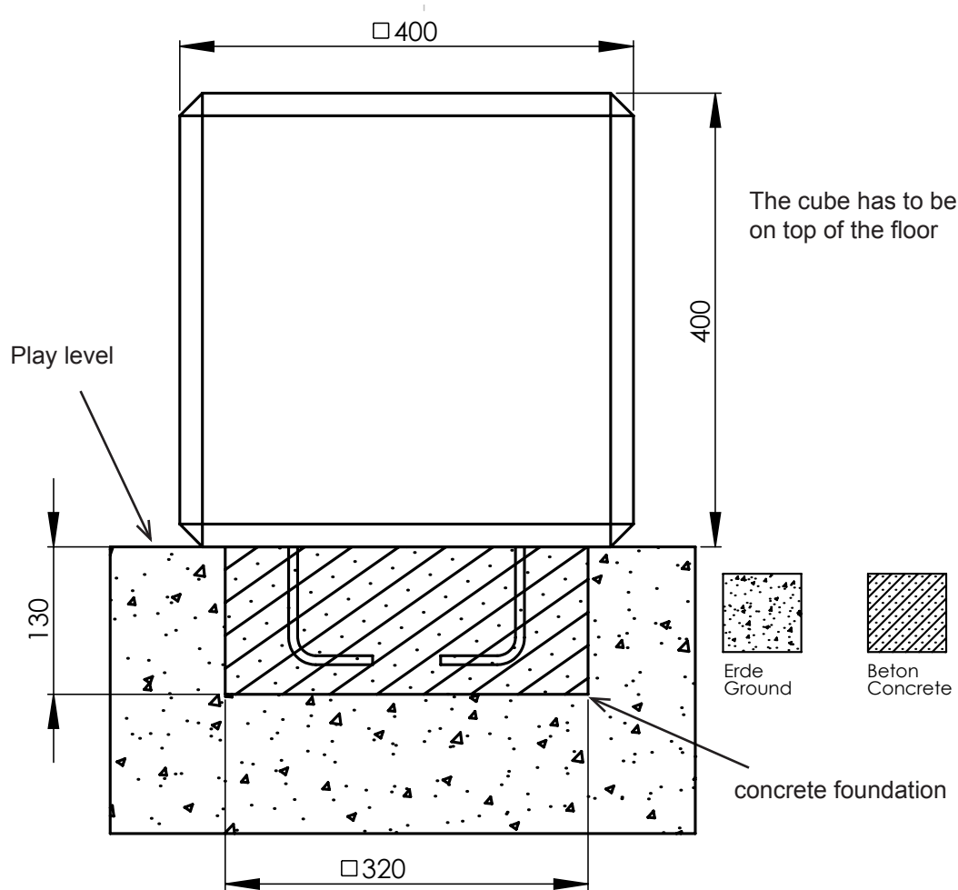
Diagram 2: Side view with dimension details „quadro“
