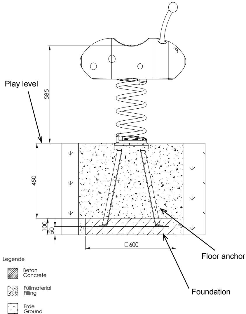
Diagram 2: Side view with dimension details „scara“
