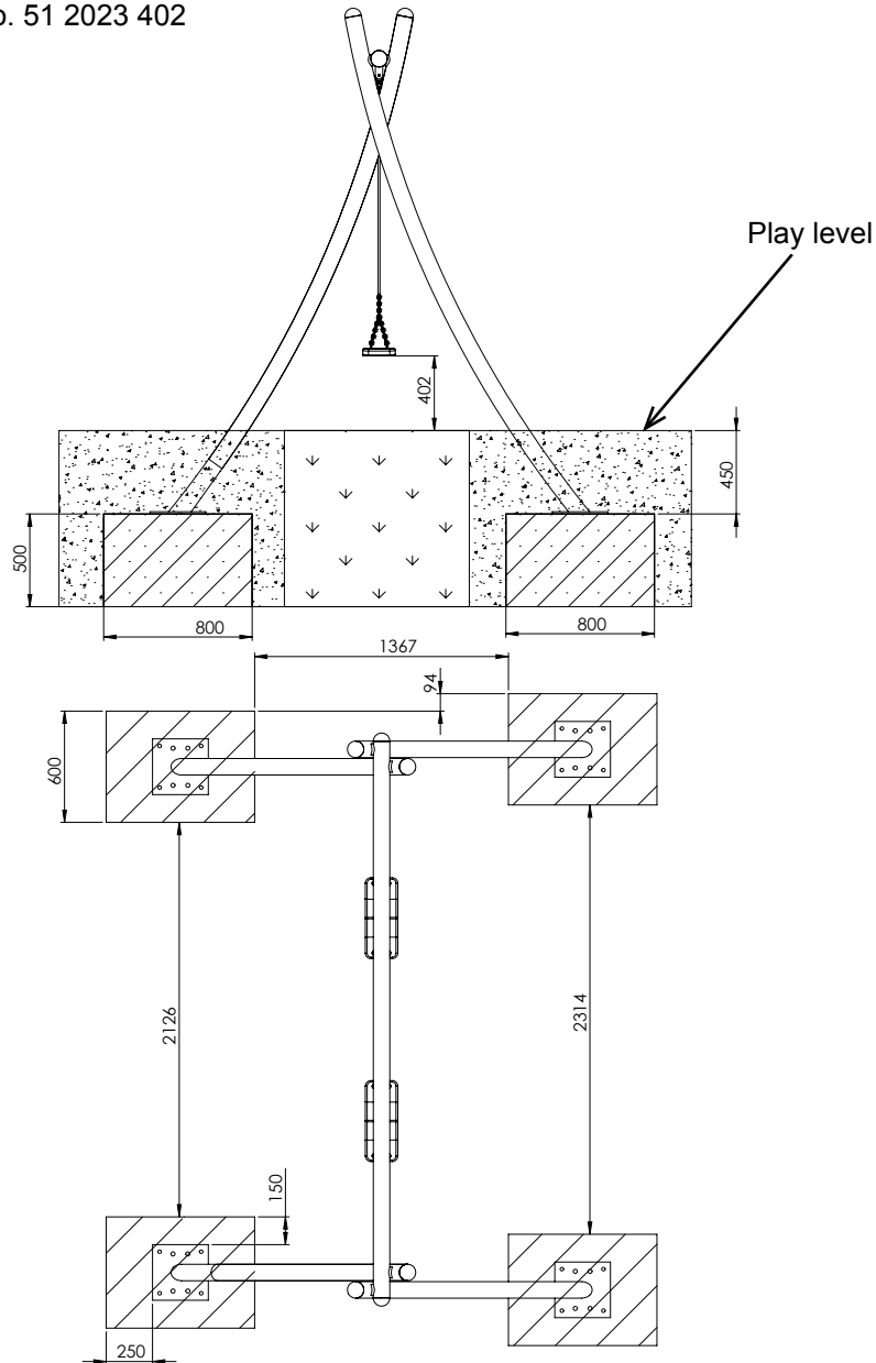
Diagram 2: Foundation plan with dimension details „vola 2“
