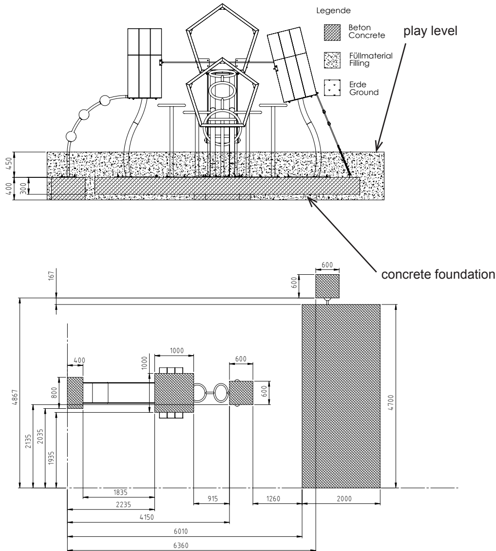
Diagram 2: Foundation plan with dimension details „sura 4a“
