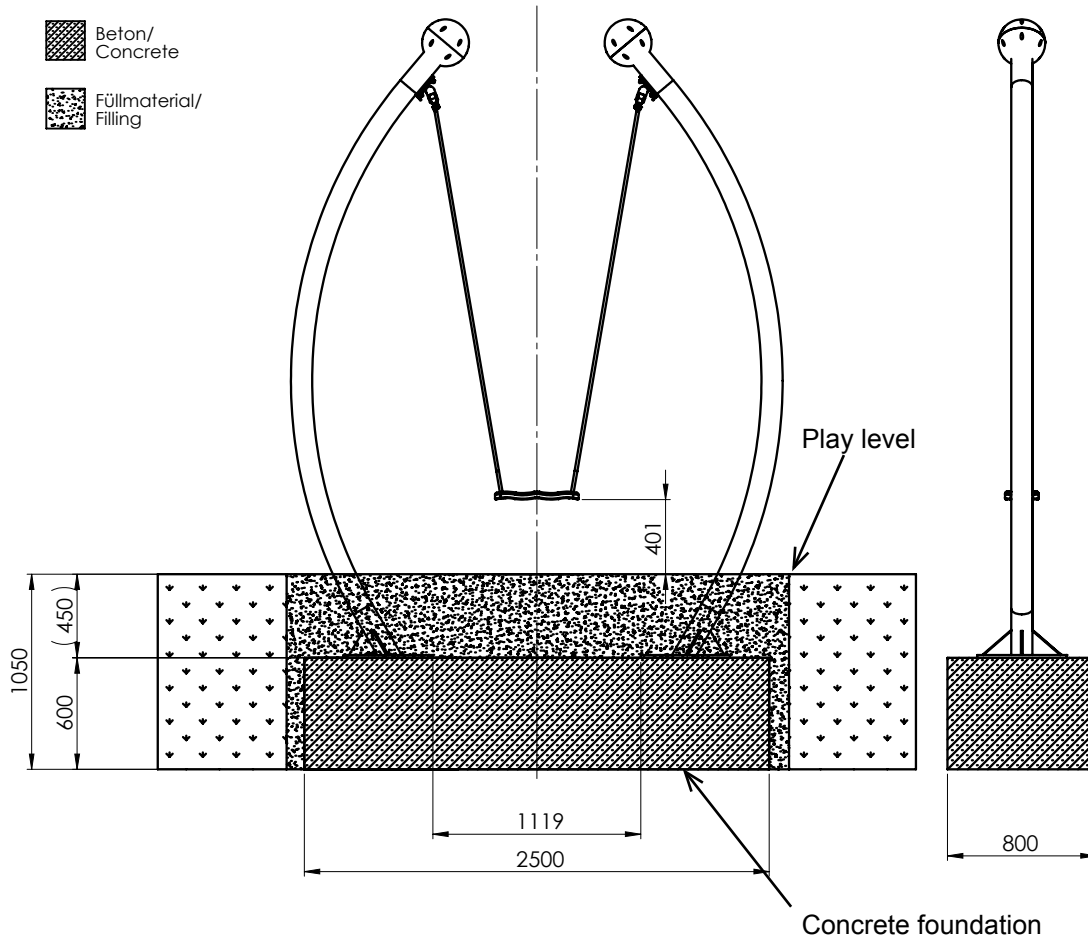
Diagram 2: Side view with dimension details „divo“
