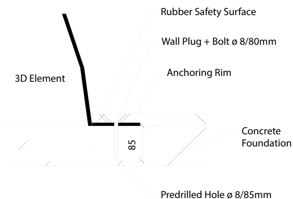
Element anchoring detail
