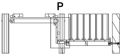
E-E ( 1/50 )
