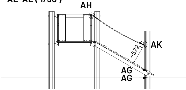
AE-AE ( 1/50 )
