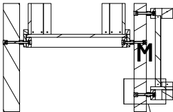
L-L ( 1/50 )
