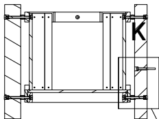
J-J ( 1/50 )
