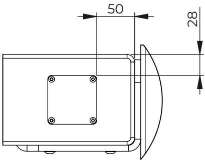
DETAIL A 1:5
