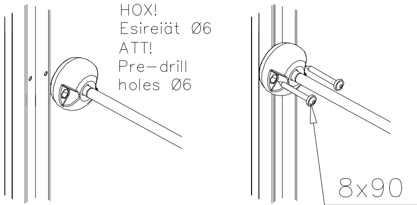
DET 5 Alternative change the height of the rope
