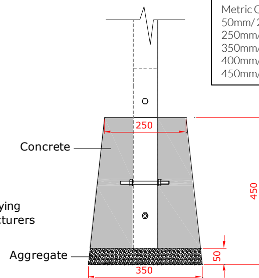
4 Fix instrument to Ground fix post using M10 bolt and Barrel Nut and use thread locking solution to prevent fixings working loose.
